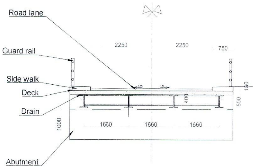
BRIDGE TRANSVESAL SECTION
