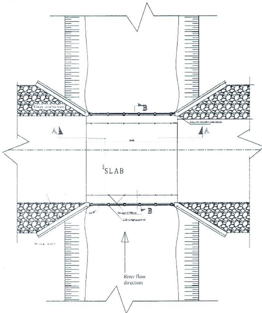
LAYOUT PLAN
